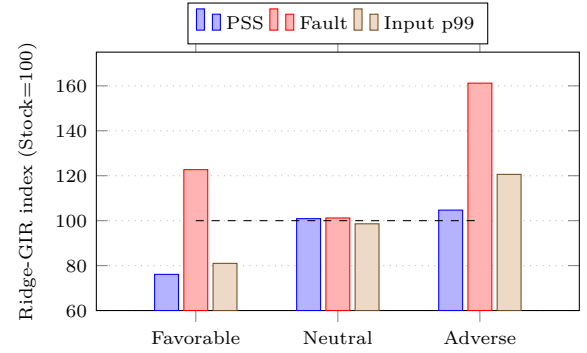
Fig. 1. Cross-regime robustness of the coordinated learned policy ( Ridge-GIR ). Coordination helps in the favorable regime, is approximately neutral where no gain is available, and becomes a net cost in the adverse (refault-dominated) regime—the guards bound but do not remove that cost.
