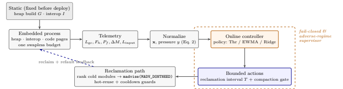
Fig. 1. SAGE-MM runtime composition and the narrow online action space (reclamation interval T and compaction gate). Static interventions (heap build G , interop I ) sit upstream and reduce the pressure presented to the controller; only the control path adapts online. Per-interval telemetry is normalized into a dimensionless pressure, the interchangeable policy emits the two bounded actions, and the reclamation path issues advise (MADV_DONTNEED) through the conservative native helper under the hot-reuse and cooldown guards. The dashed band marks the policy-independent fail-closed and adverse-regime supervisory guards.
