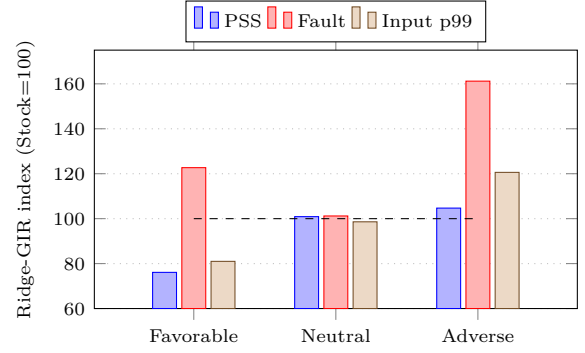
Fig. 4. Cross-regime robustness of the coordinated learned policy ( Ridge-GIR ). Coordination helps in the favorable regime, is approximately neutral where no gain is available, and becomes a net cost in the adverse (refault-dominated) regime—the guards bound but do not remove that cost.
