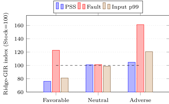
Fig. 1. Cross-regime robustness of the coordinated learned policy (Ridge-GIR). Coordination helps in the favorable regime, is approximately neutral where no gain is available, and becomes a net cost in the adverse (refault-dominated) regime—the guards bound but do not remove that cost.
