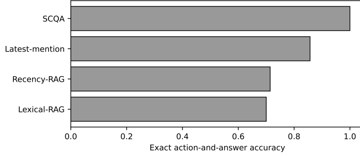
Fig. 3 Oracle-state diagnostic accuracy. The result demonstrates that the specified invariants are executable. It does not estimate end-to-end LLM accuracy because situation variables are supplied rather than inferred.
