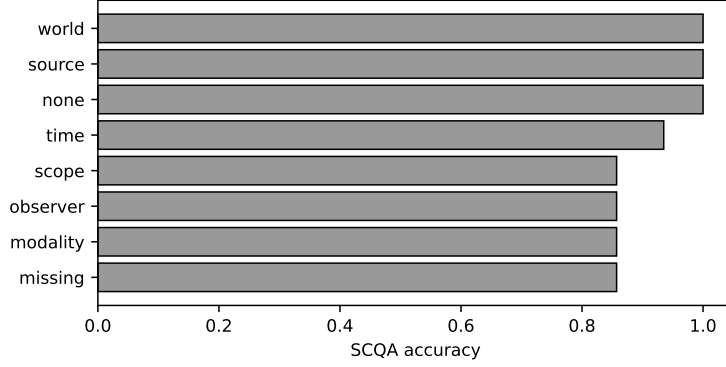
Fig. 5 Oracle-state component ablations. Each removed variable recovers the predicted category-specific failure, providing a causal software diagnostic.
