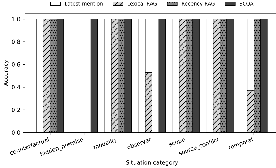
Fig. 4 Accuracy by diagnostic category. Each category isolates one applicability variable, enabling mechanism-level failure localization.
