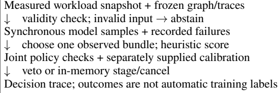
Figure 1: REST decision path. The telemetry demo is marked invalid for end-to-end latency, so it abstains. Versioned objective preferences and automatic graph/calibration refresh are future requirements; the separate per-thread experiment uses a fixed latency objective and frozen artifacts.
