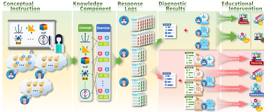
Fig. 1: A toy example of typical CD and mastery-fluency CD.
