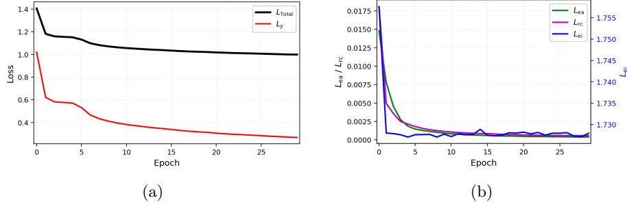
Fig. 5: Loss curves of (a) L_{Total} , L_y , and (b) L_{ei} , L_{ea} , L_{rc} .
