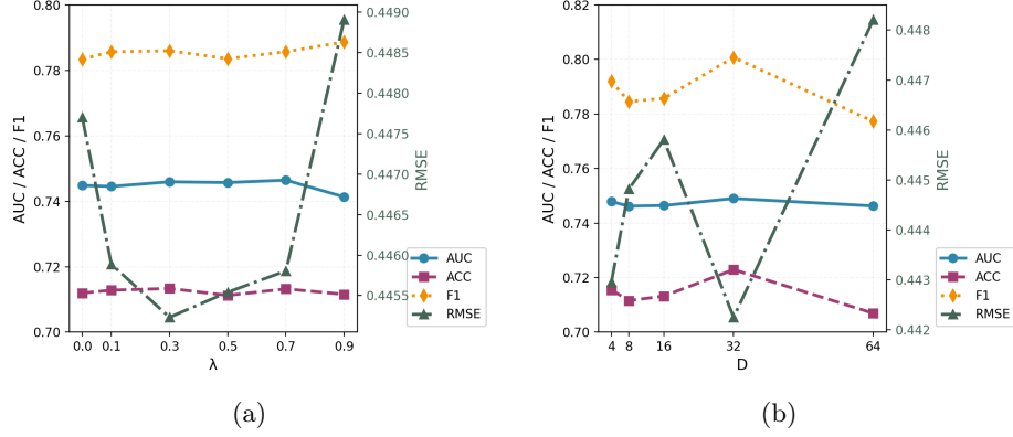
Fig. 4: Sensitivity analysis of (a) weight \lambda and (b) dimension D of latent fluency state \mathbf{z}_{i,k} .
