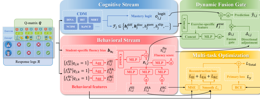
Fig. 2: The overall architecture of MFCD.
