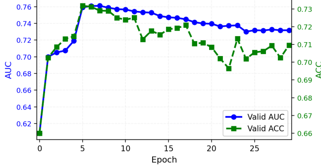
Fig. 6: Validation AUC and ACC curves.
