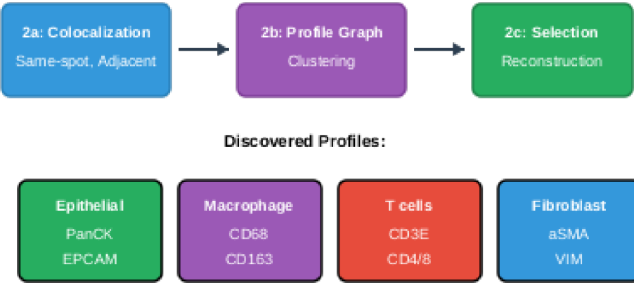
Automatic marker-to-cell-type profile assembly
