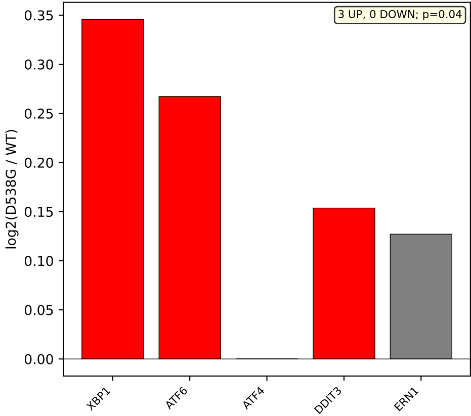
UPR Markers in MCF7-D538G
