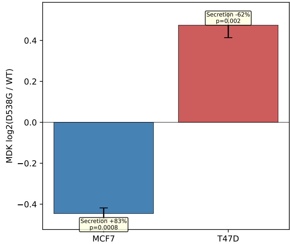
MDK mRNA Anti-correlation
