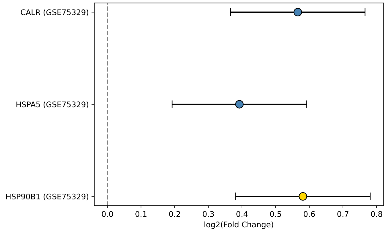
C. Forest Plot: Chaperone Response to ER Knockdown
