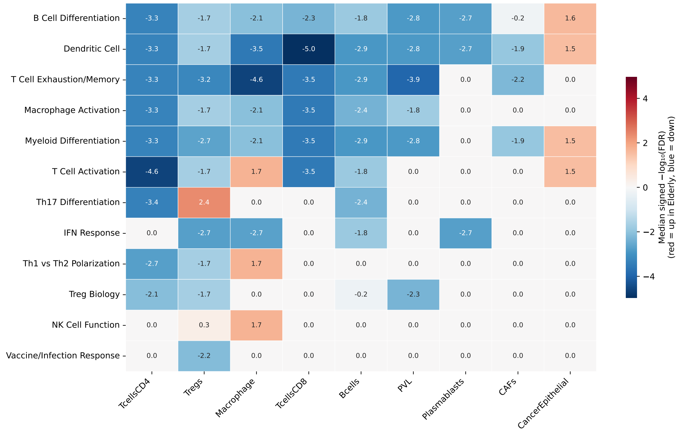
ImmuneSigDB (MSigDB C7): Immune Themes Elderly vs Young (Pseudobulk DESeq2, \geq 2 significant sets per theme)
