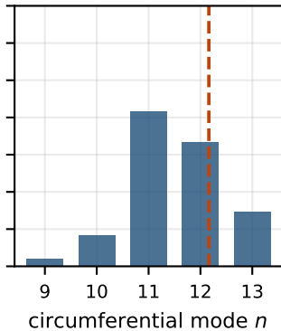
R/t = 200, L/R = 1.0
