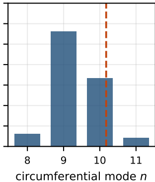
R/t = 140, L/R = 1.0
