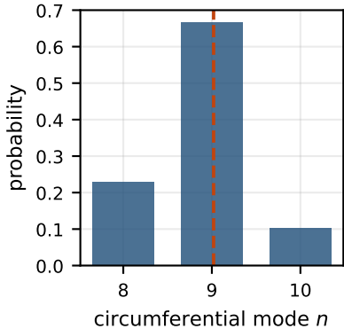
R/t = 110, L/R = 1.0
