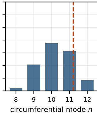
R/t = 170, L/R = 1.0
