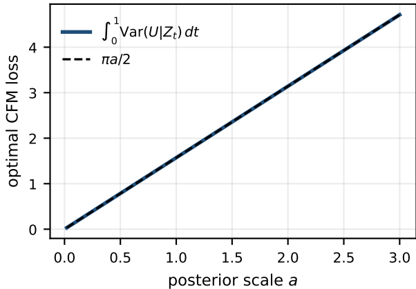
(a) loss floor is linear in a
