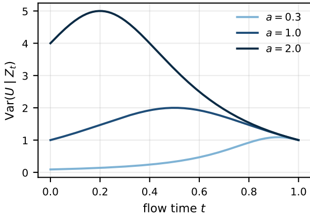
(b) irreducible conditional variance
