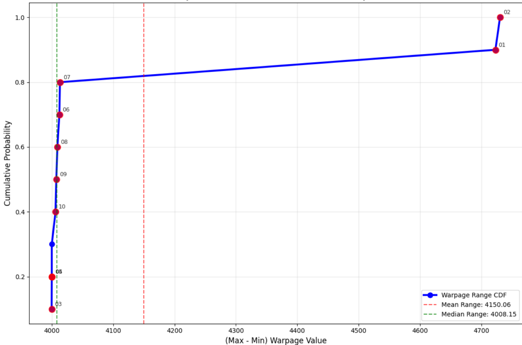
Cumulative Distribution of Warpage Ranges (X-axis: Max-Min values across files)
