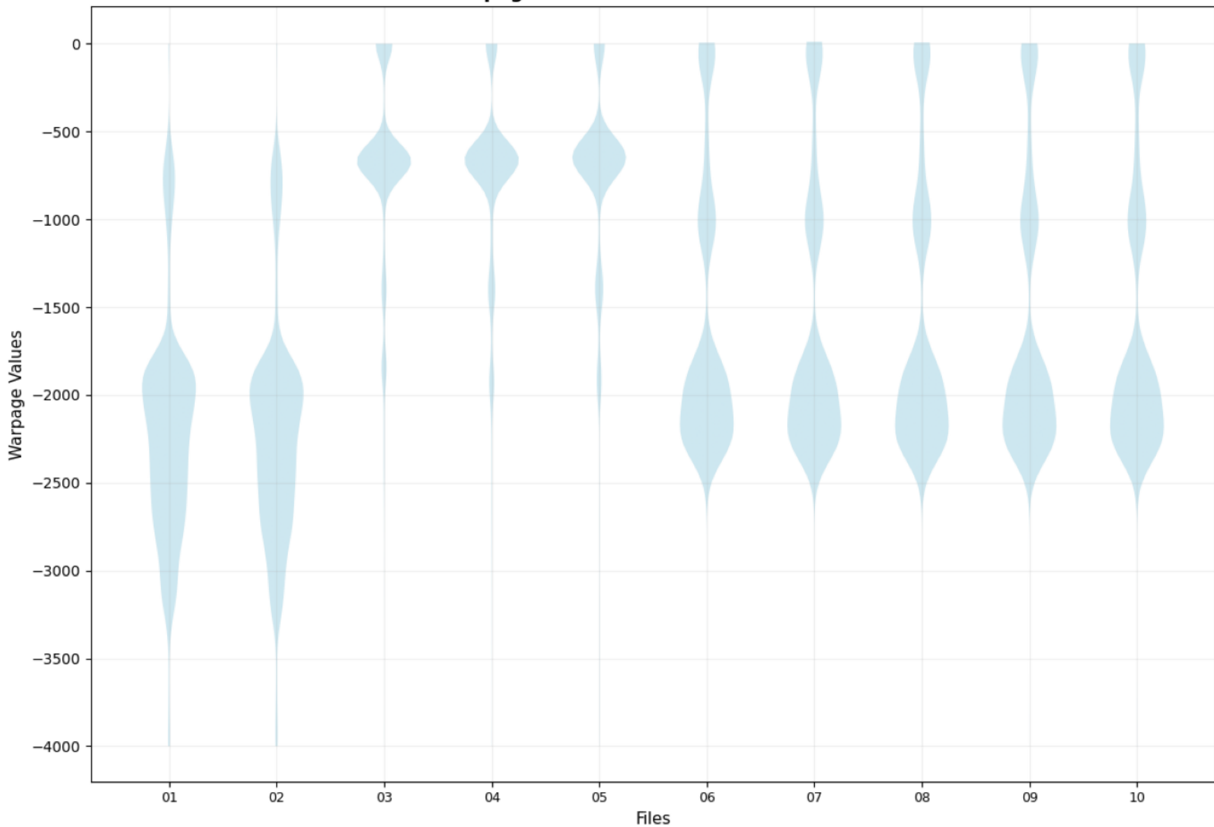
Warpage Distribution - Fast Violin Plots
