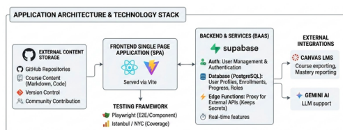
Figure 1. MasteryLS system architecture: GitHub stores canonical course content while a managed backend handles operational data and mediates AI and gradebook integrations.
