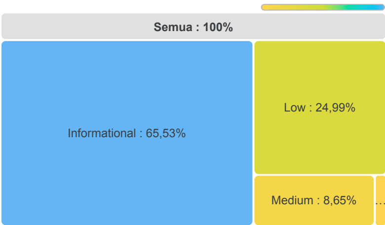
Threat Category
