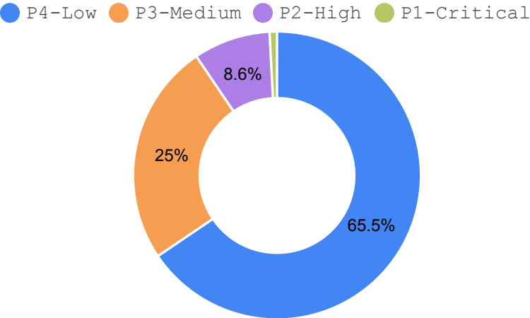
Priority Distribution
