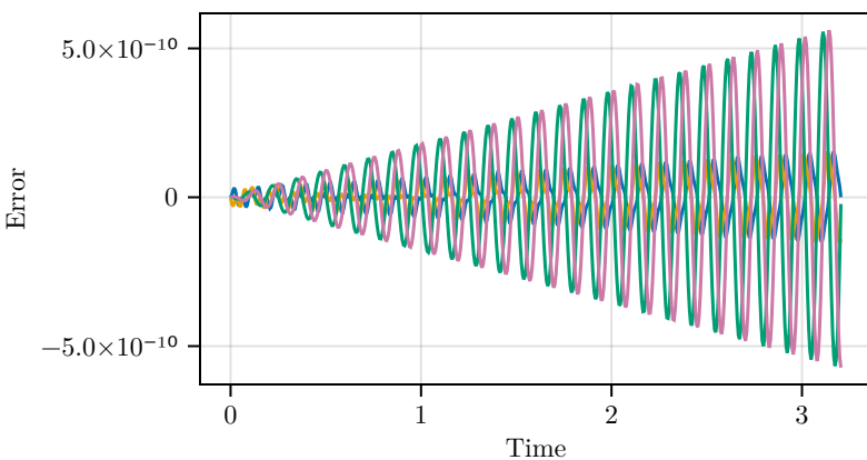
Lab frame : Filon error ( \omega \neq 0 ) - ( \omega = 0 )
