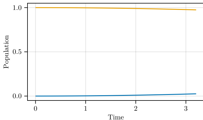
Rotating frame (RWA) : populations
