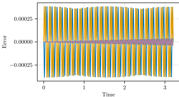
Error : rotating frame (in lab) vs lab frame
