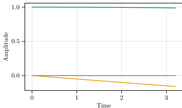
Error : rotating frame (in lab) vs lab frame
