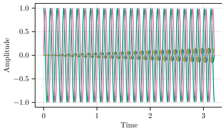
Rotating frame (RWA) : complex amplitudes
