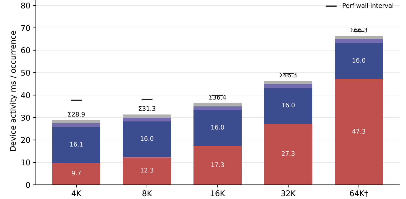
AR step · module execution time
