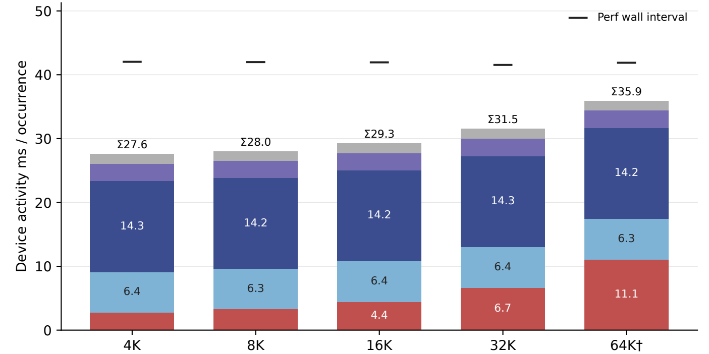
AR step · module execution time
