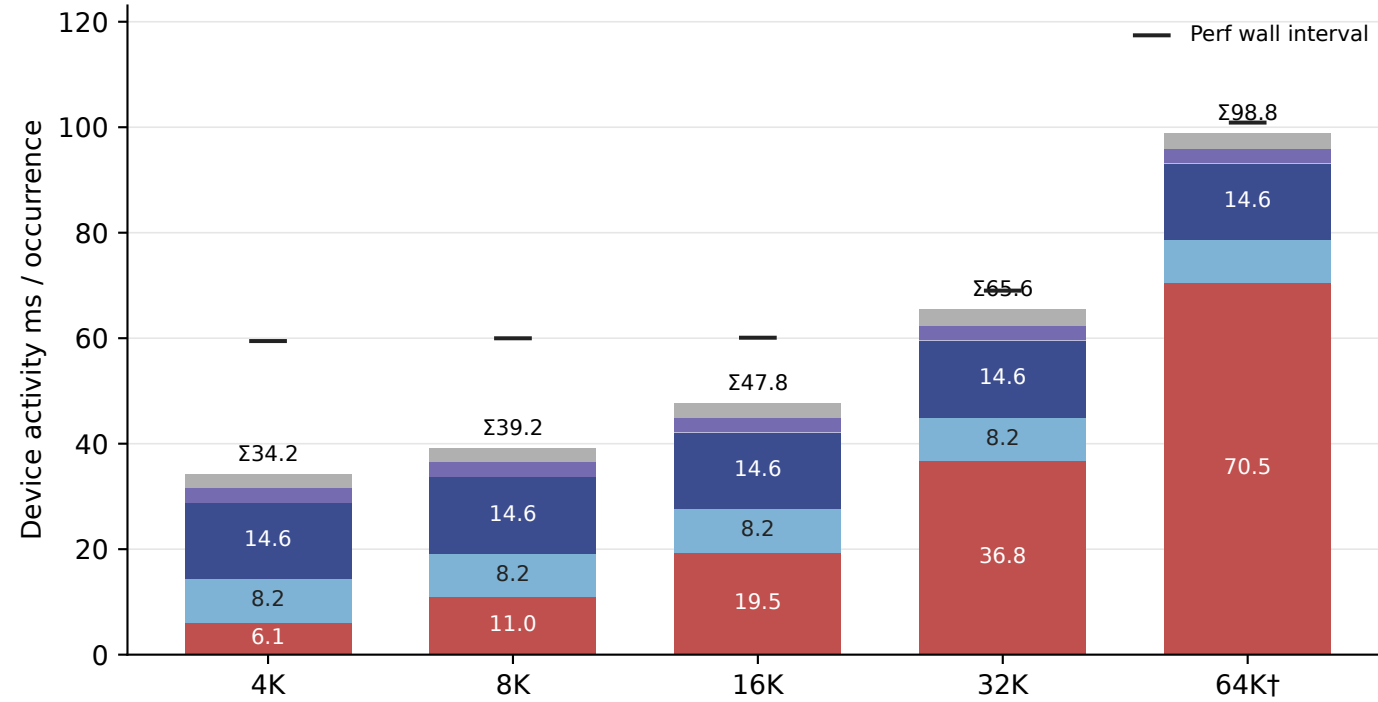
DFlash verify · module execution time
