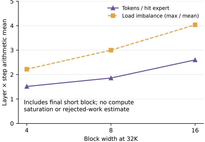
F Each hit expert still receives few tokens
