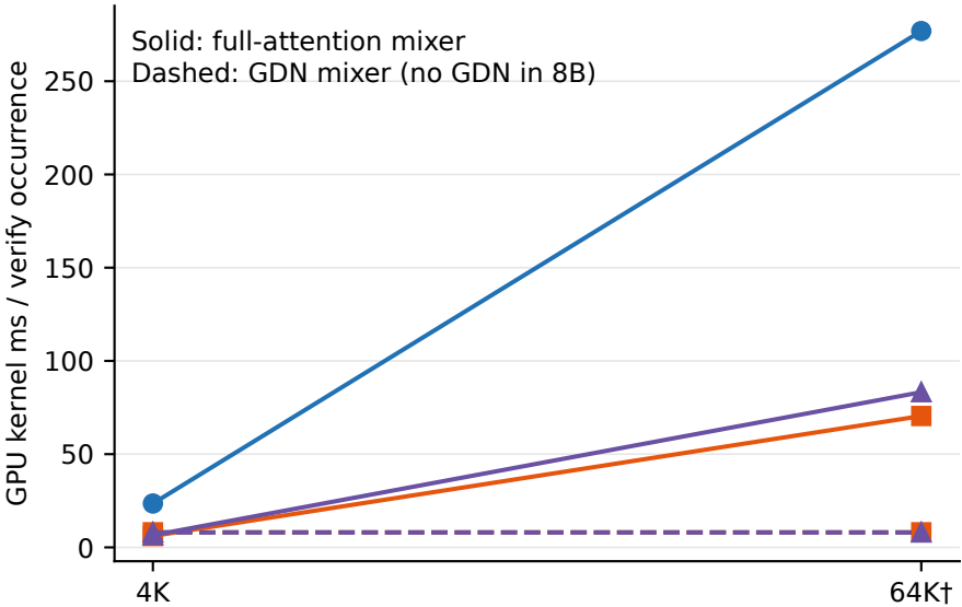
B Full-attention mixer vs GDN mixer
