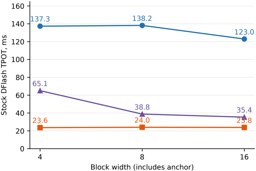
D 32K block sweep: latency per output token
