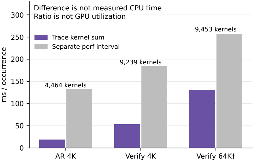
C 35B GPU kernel sums and perf intervals
