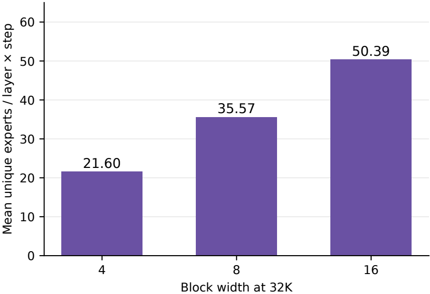
E 35B: expert union broadens with block width
