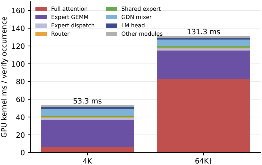
A 35B verify GPU kernel breakdown
