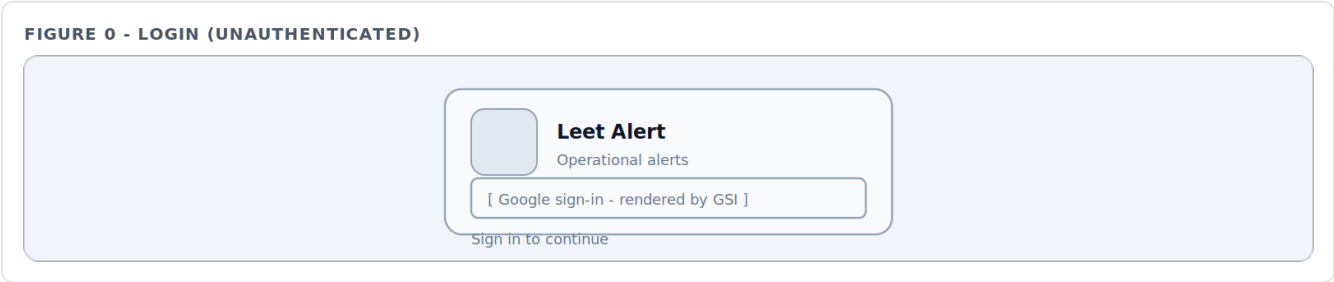
Figure 0 — Login
