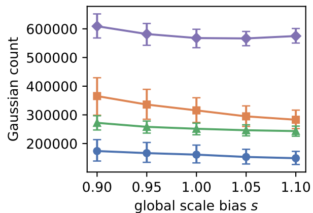
Gaussian count vs. s
