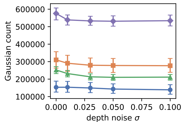
Gaussian count vs. \sigma
