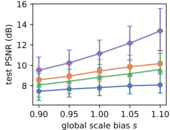
PSNR vs. s (noise fixed at 0)
