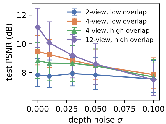
PSNR vs. \sigma (scale bias fixed at 1.0)
