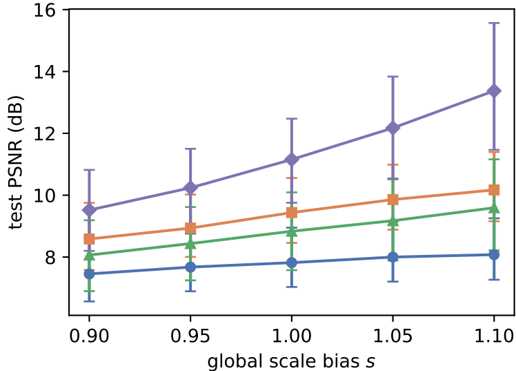
PSNR vs. s (noise fixed at 0)
