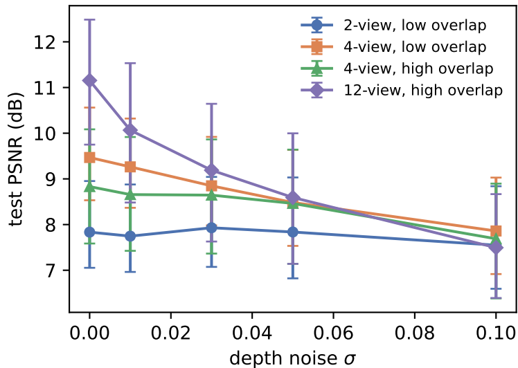
PSNR vs. \sigma (scale bias fixed at 1.0)
