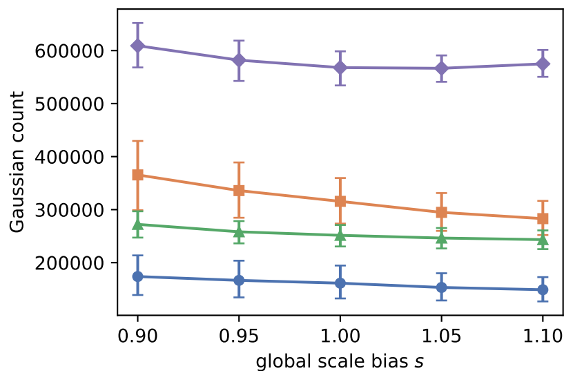
Gaussian count vs. s
