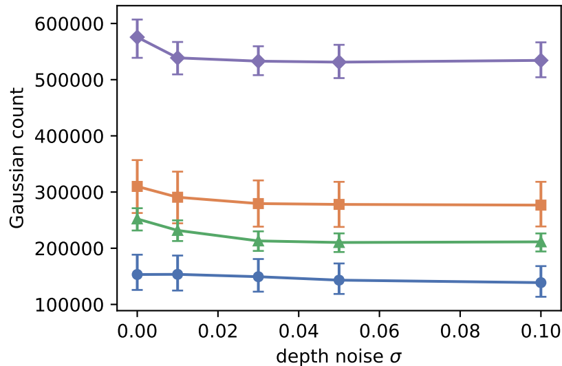
Gaussian count vs. \sigma
