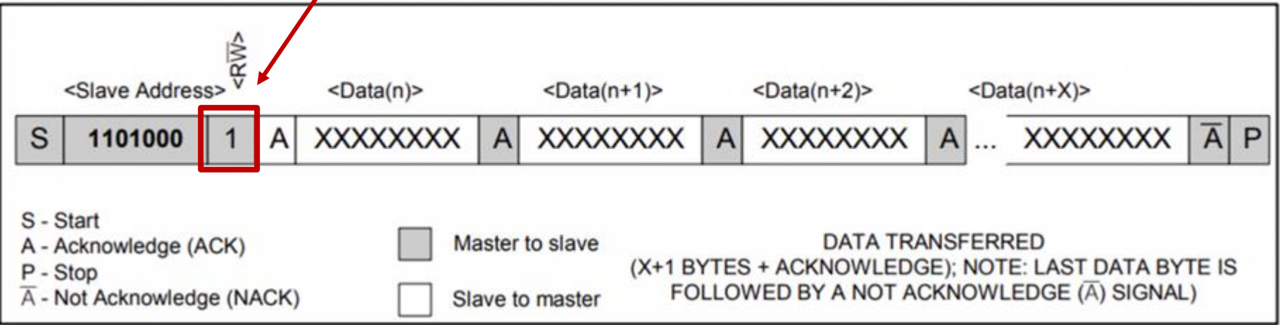
Figure 5. Data Read—Slave Transmitter Mode
