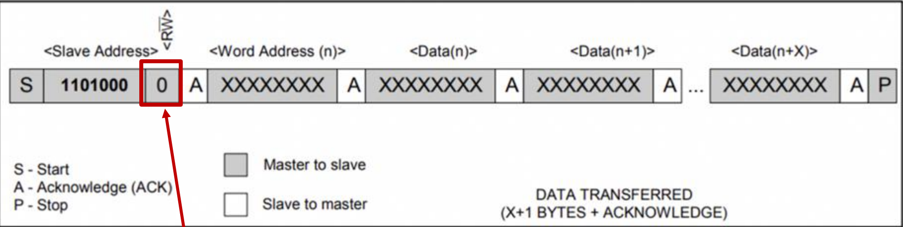
Figure 4. Data Write—Slave Receiver Mode
