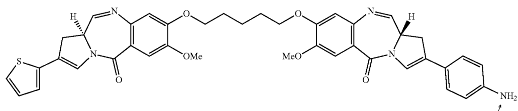
PBD Dimer 5
