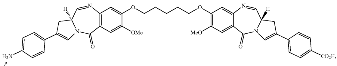
PBD Dimer 11
