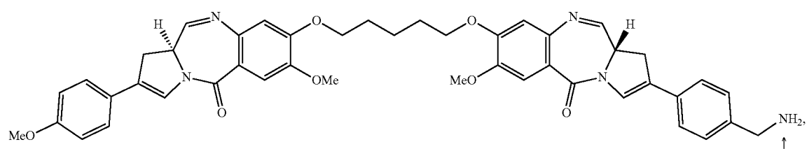
PBD Dimer 7
