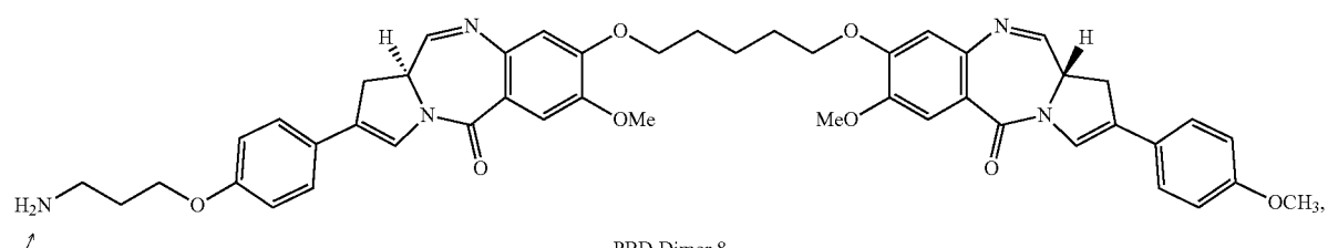
PBD Dimer 8
