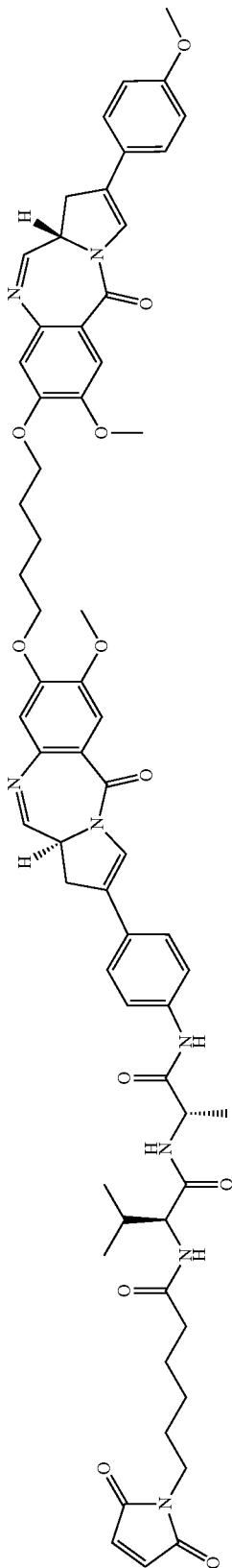
Compound 2
