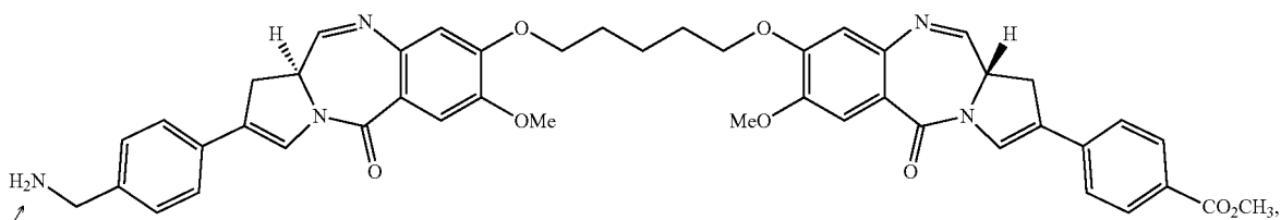
PBD Dimer 14
