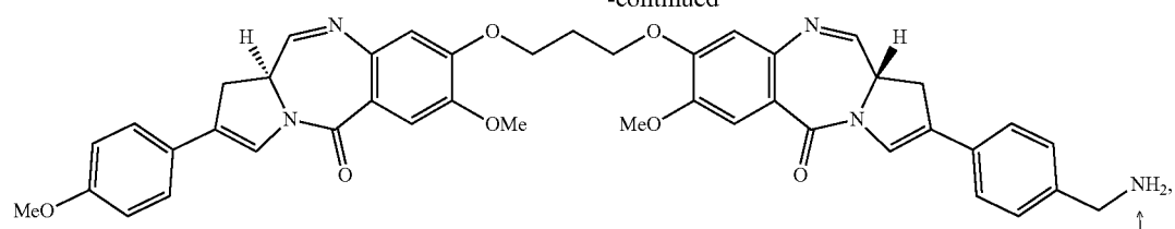
PBD Dimer 4
