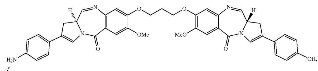
PBD Dimer 9
