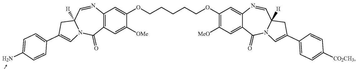
PBD Dimer 12
