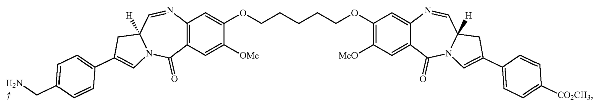
PBD Dimer 15
