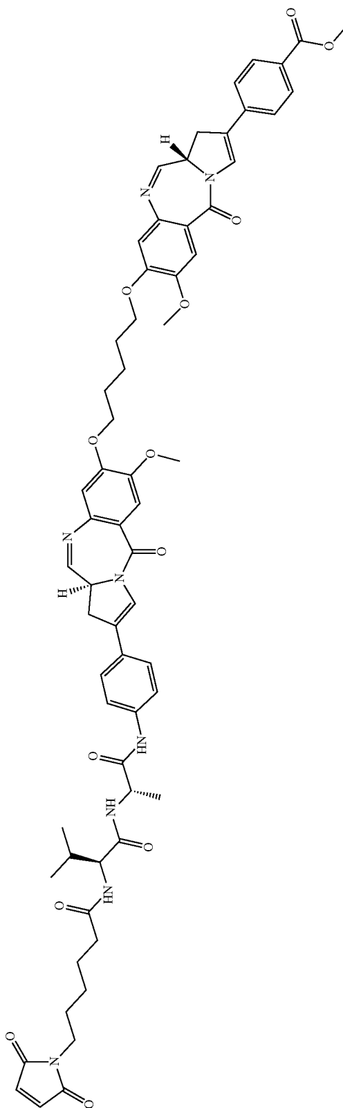
Compound 3
