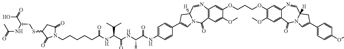
Compound 4
