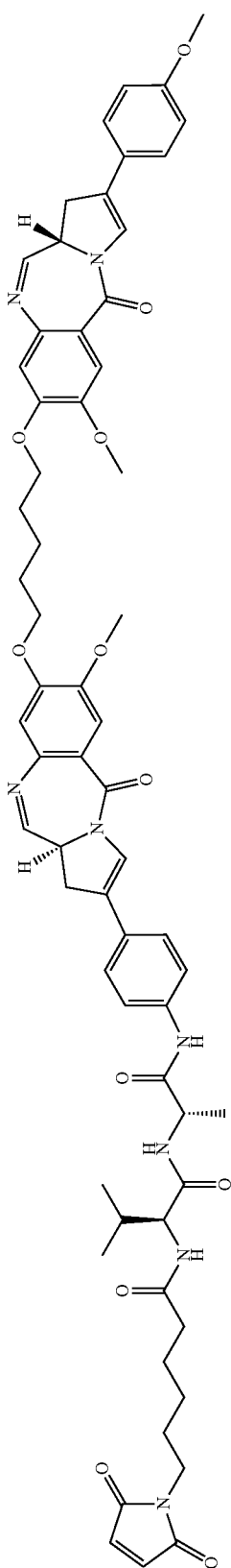
Compound 1
