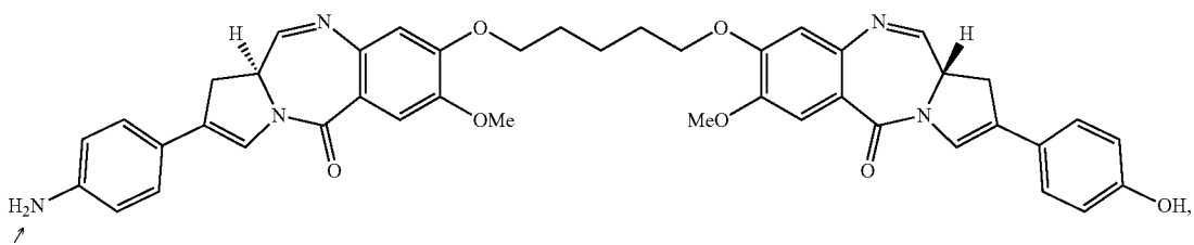
PBD Dimer 10
