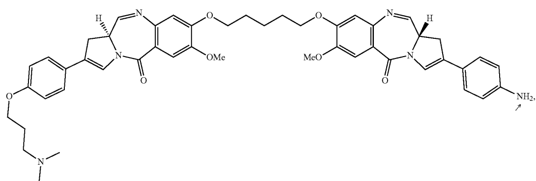
PBD Dimer 6
