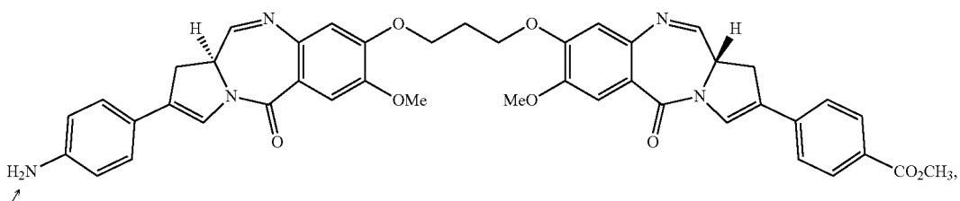
PBD Dimer 13
