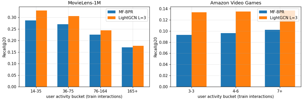
Figure 6: Recall@20 per activity bucket, corresponding to Table ??.
