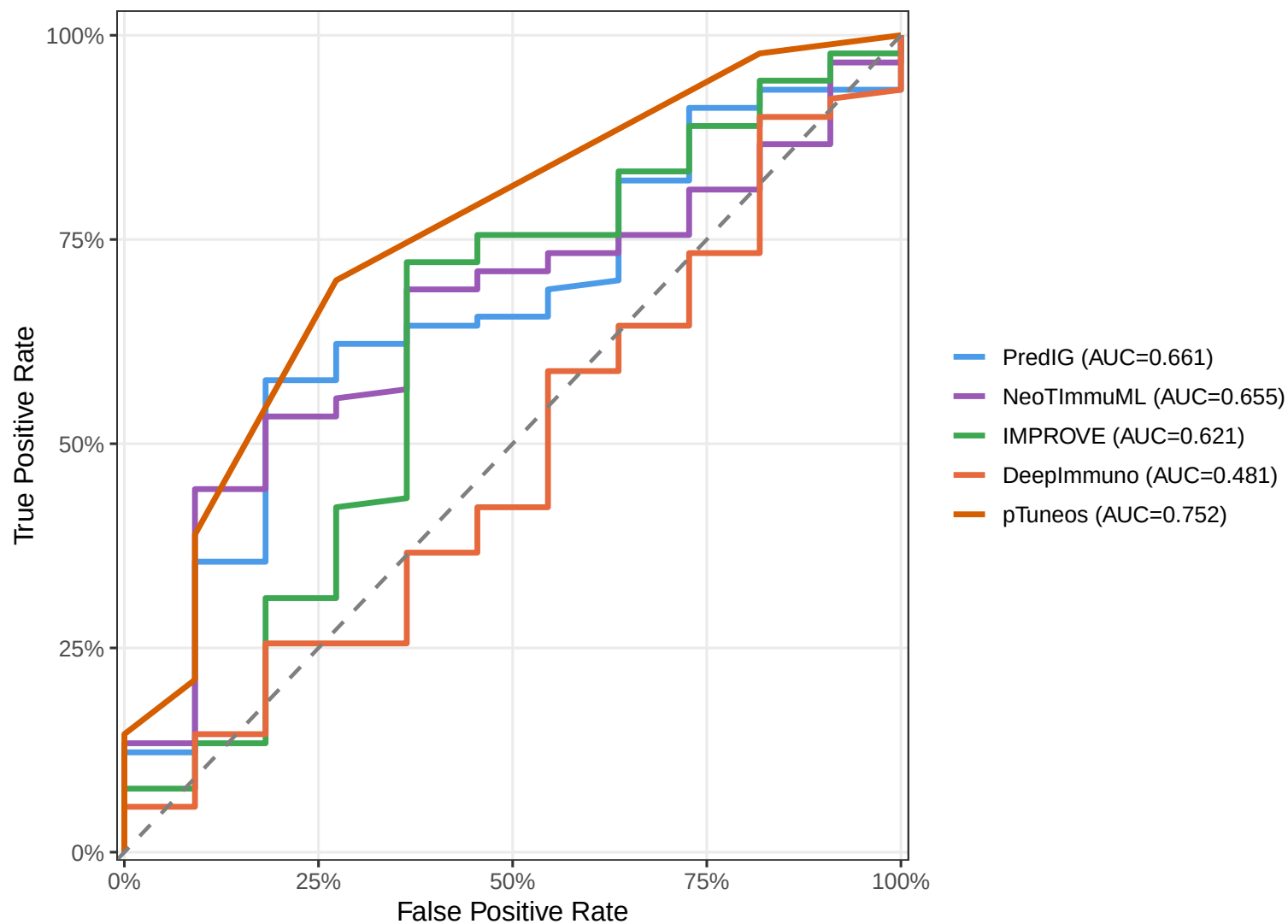
ROC Curves — DS2, ELISpot > 0, Aggregation = max
