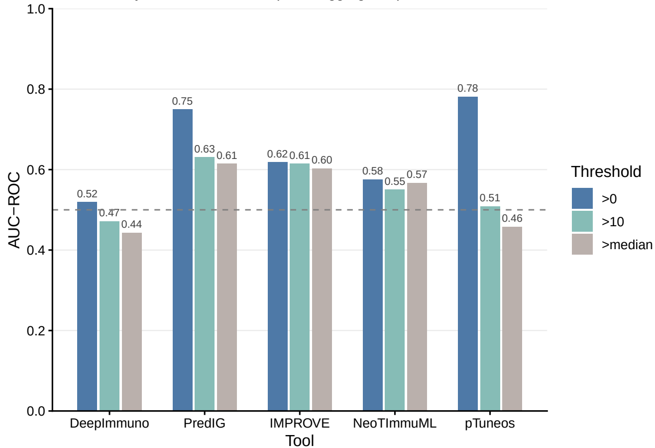
AUC-ROC by Tool and Threshold (mean aggregation)
