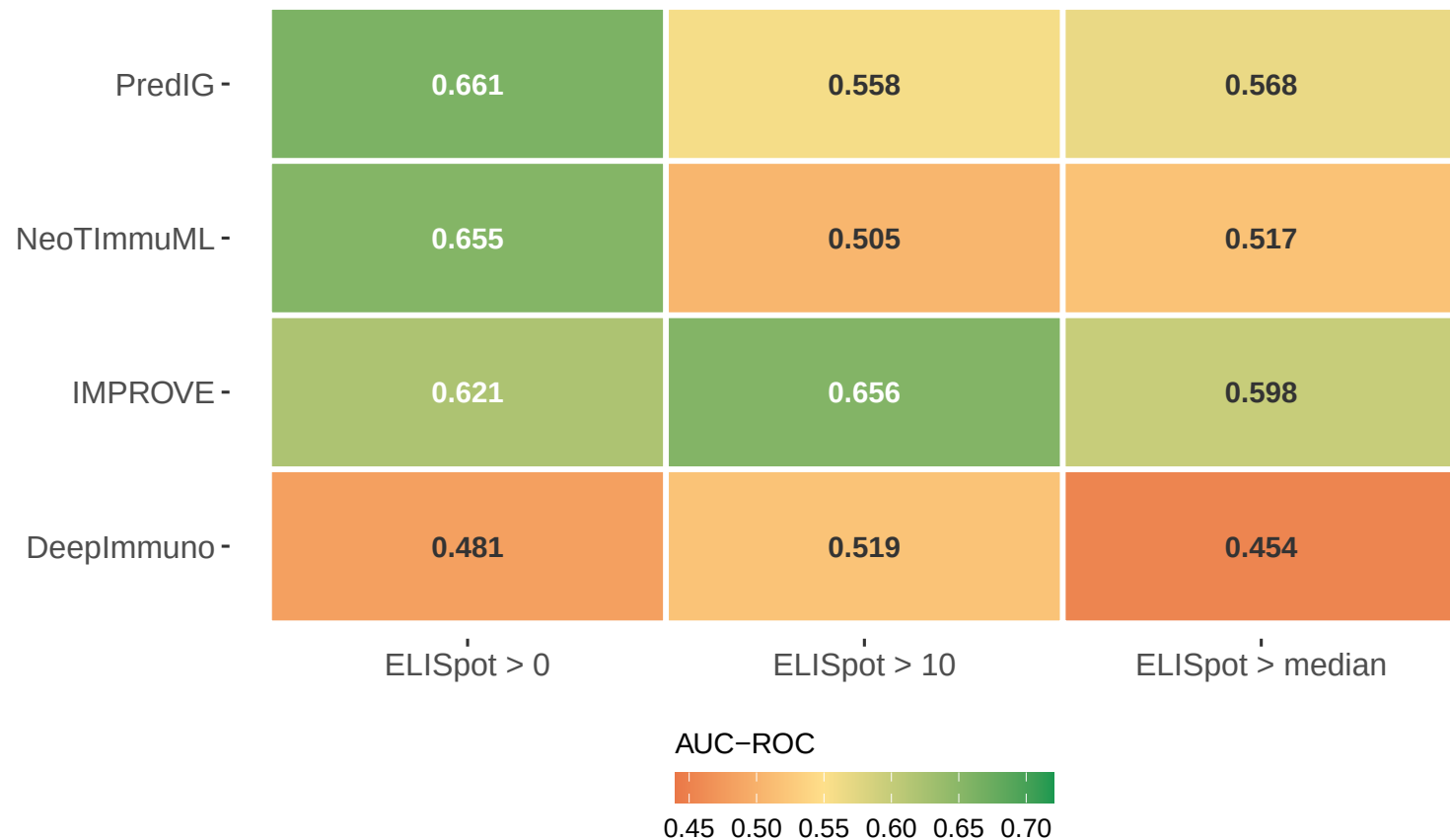
AUC-ROC Heatmap — Tool × Threshold (Aggregation = max)
