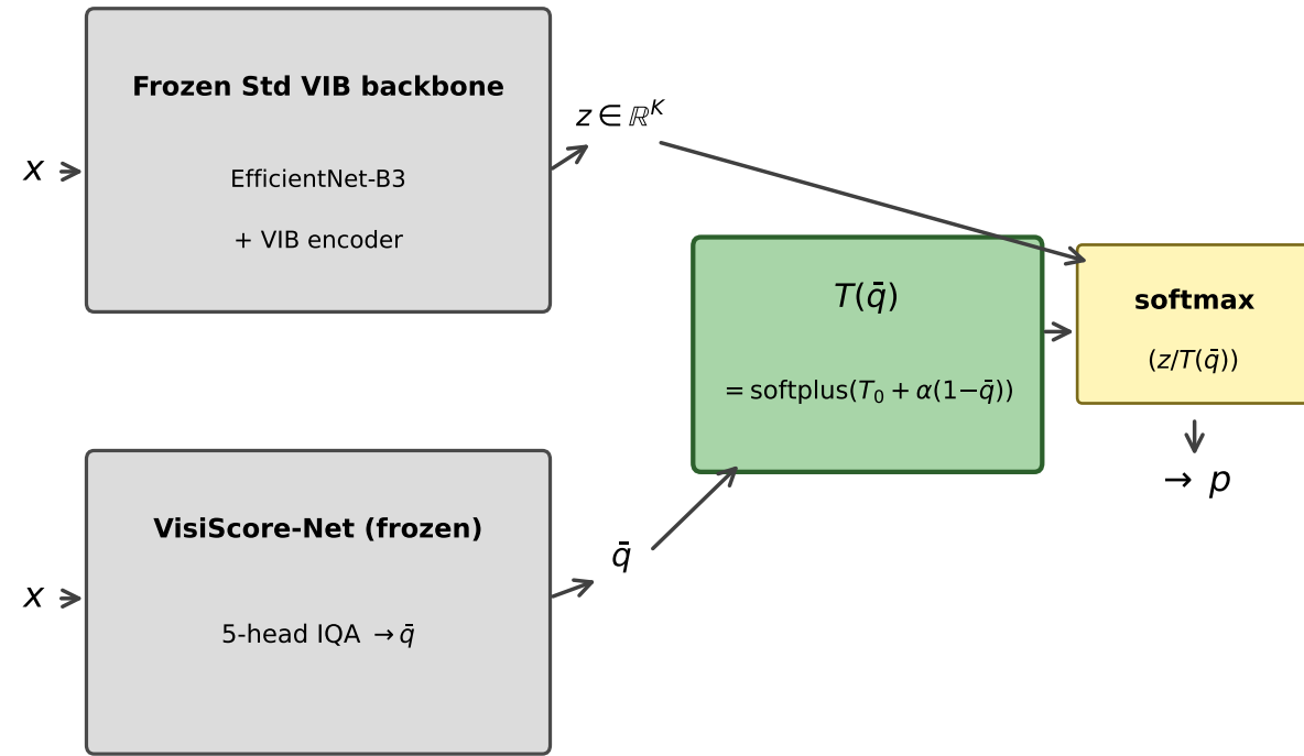
(b) QCTS architecture
