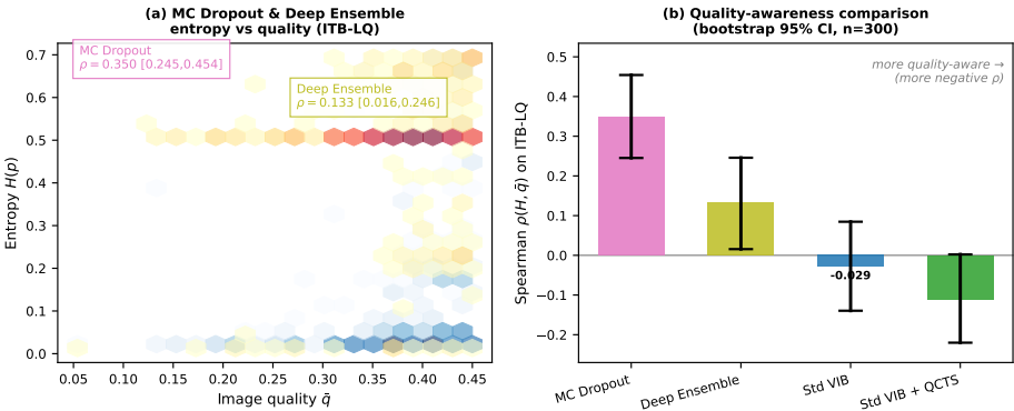
Figure S7: Entropy vs. \hat{q} scatter on ITB-LQ ( n=300 ) for four methods. MC Dropout achieves \rho = +0.350 ( p < 10^{-9} ) and Deep Ensemble \rho = +0.133 ( p=0.021 ), both positive: within the LQ stratum, these methods are more uncertain on marginally better-quality images — quality-oblivious at the individual-prediction level. Std VIB + QCTS achieves \rho = -0.112 (one-sided p=0.054 ), consistently more negative than any other method in the LQ stratum.
