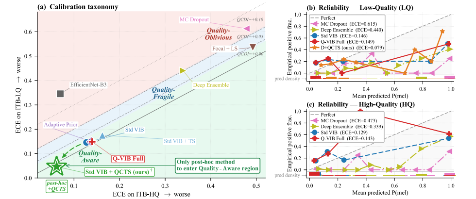
Figure S1: Quality-conditioned calibration problem. (a) Taxonomy: each baseline (and QCTS) placed by HQ ECE ( x ) vs. LQ ECE ( y ); the dashed diagonal is QCDI = 0 and the three shaded bands mark the regimes of §?? of the main paper. (b,c) Reliability diagrams for four representative methods plus QCTS, conditioned on ITB-LQ and ITB-HQ; the bottom density strip indicates where each method’s predictions concentrate. Originally main Fig. 3; moved to supplementary in this version.
