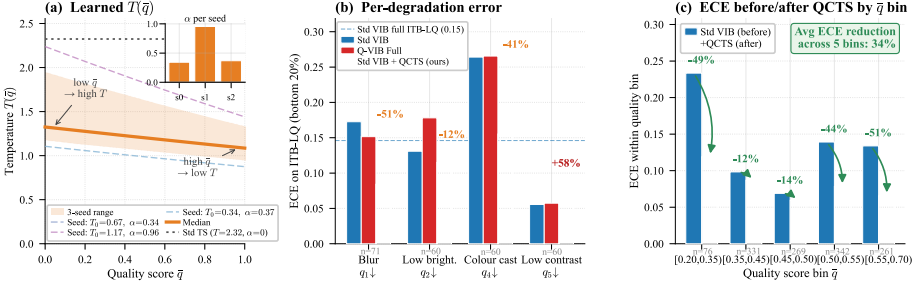
Figure S2: QCTS solution and per-bin effect. (a) Learned T(\bar{q}) across three seeds (dashed) with the median (solid) and 16/84% band; the dotted reference is standard TS ( \alpha=0 ). All seeds discover \alpha > 0 (inset). (b) Per-degradation ECE on ITB-LQ samples in the bottom 20th percentile of each quality dimension. (c) ECE before vs. after QCTS by quality bin. Originally main Fig. 4; moved to supplementary in this version.
