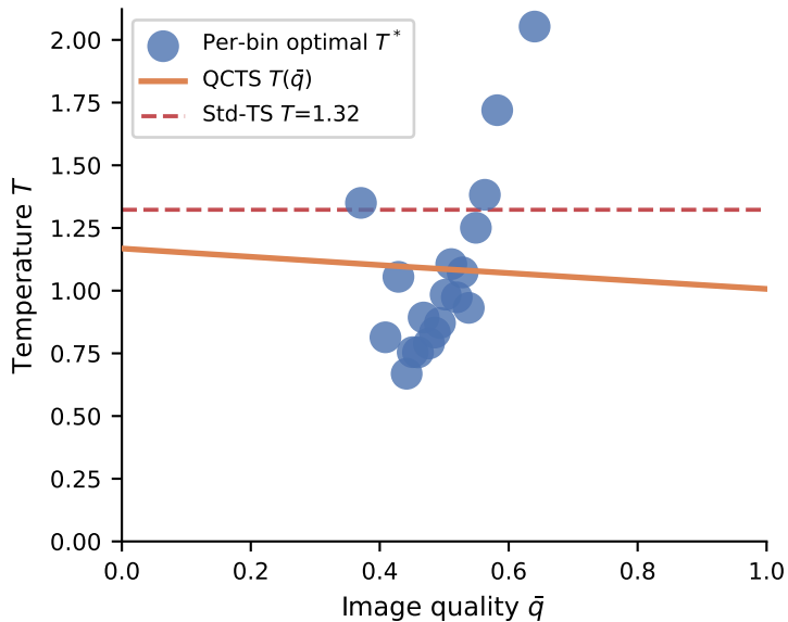
ResNet-50
