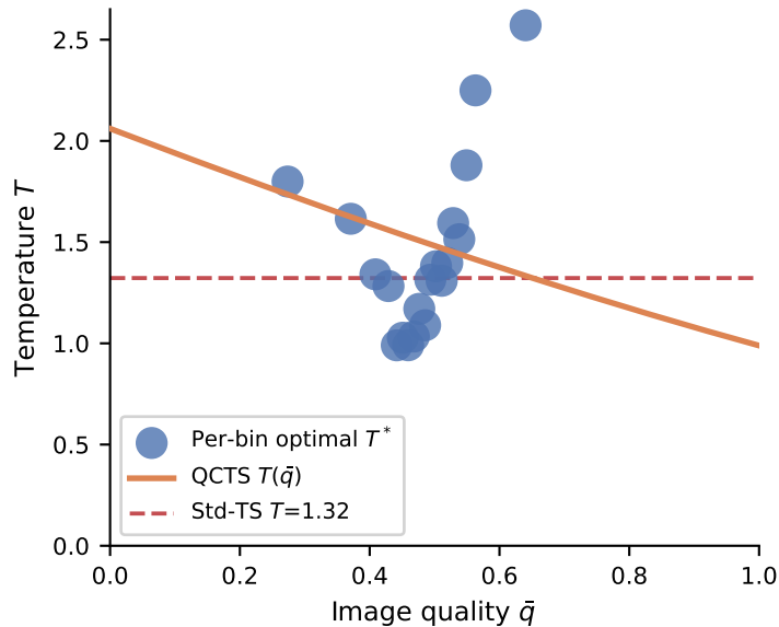
ViT-Tiny (DeiT)
