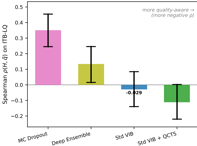
(b) Quality-awareness comparison (bootstrap 95% CI, n=300)
