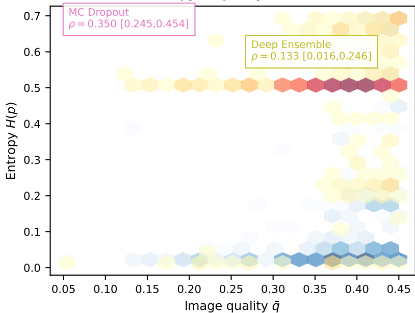
(a) MC Dropout & Deep Ensemble entropy vs quality (ITB-LQ)
