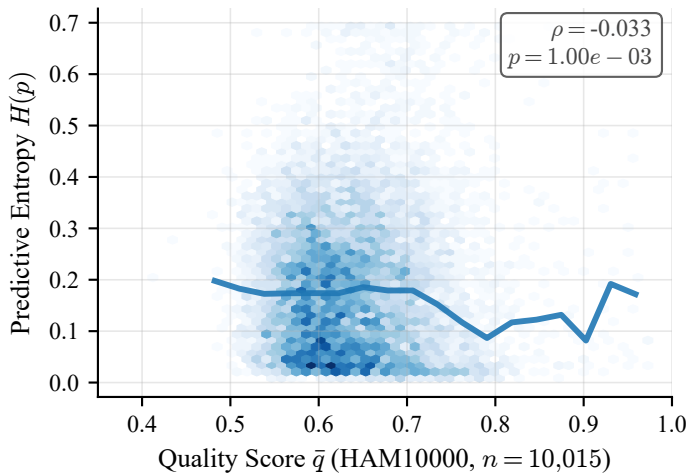
Std VIB
