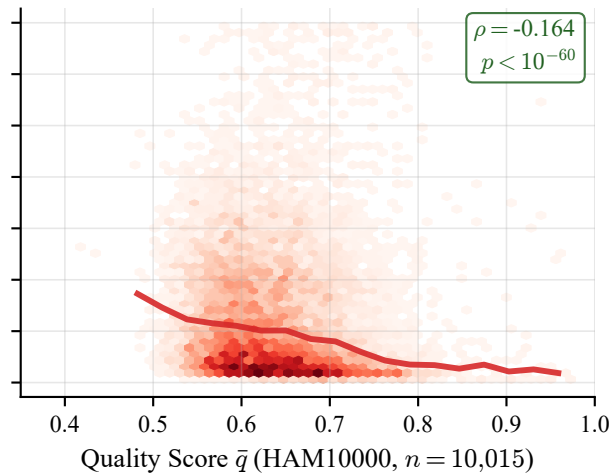
Q-VIB Full
