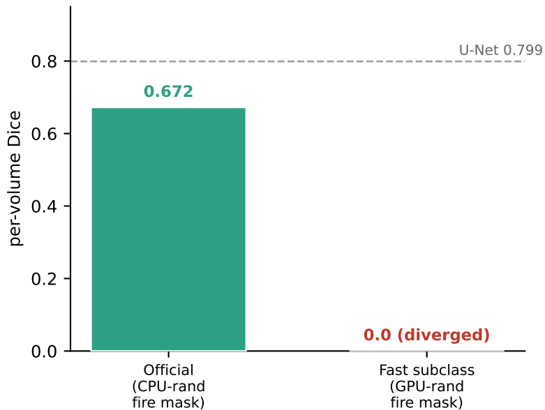
(a) RNG-stream change (mathematically equivalent)
