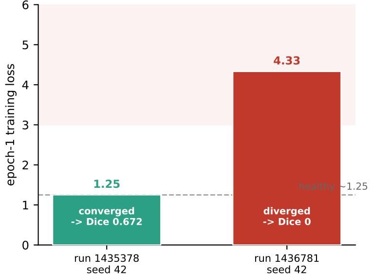
(b) same seed, same code (cuDNN FP nondeterminism)
