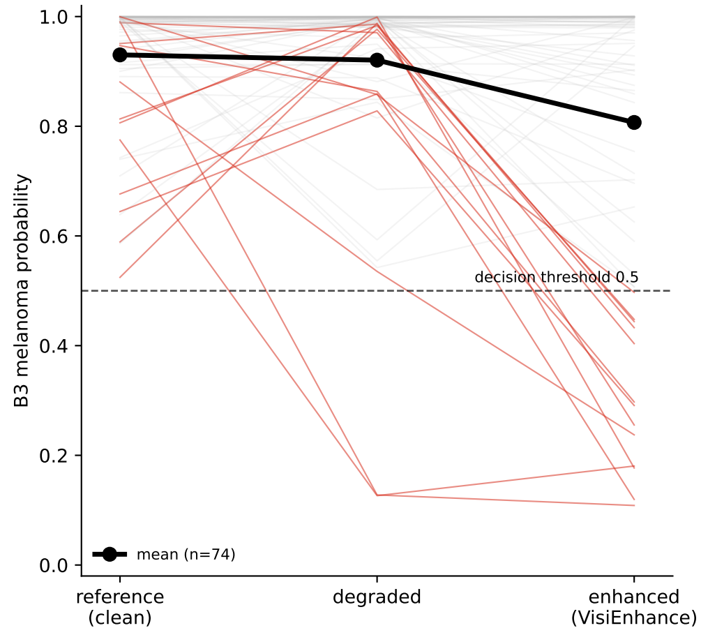
(a) Enhancement suppresses melanoma confidence mean \bar{p} 0.93 \rightarrow 0.81 (ref \rightarrow enh); 13/74 true melanomas flip below 0.5
