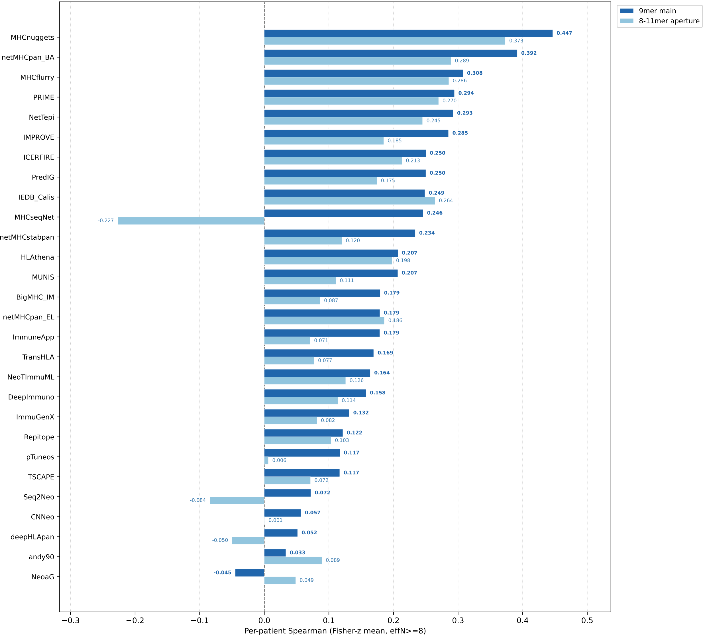
Per-patient Spearman: 9mer main vs 8-11mer variable-window aperture (effN>=8)
