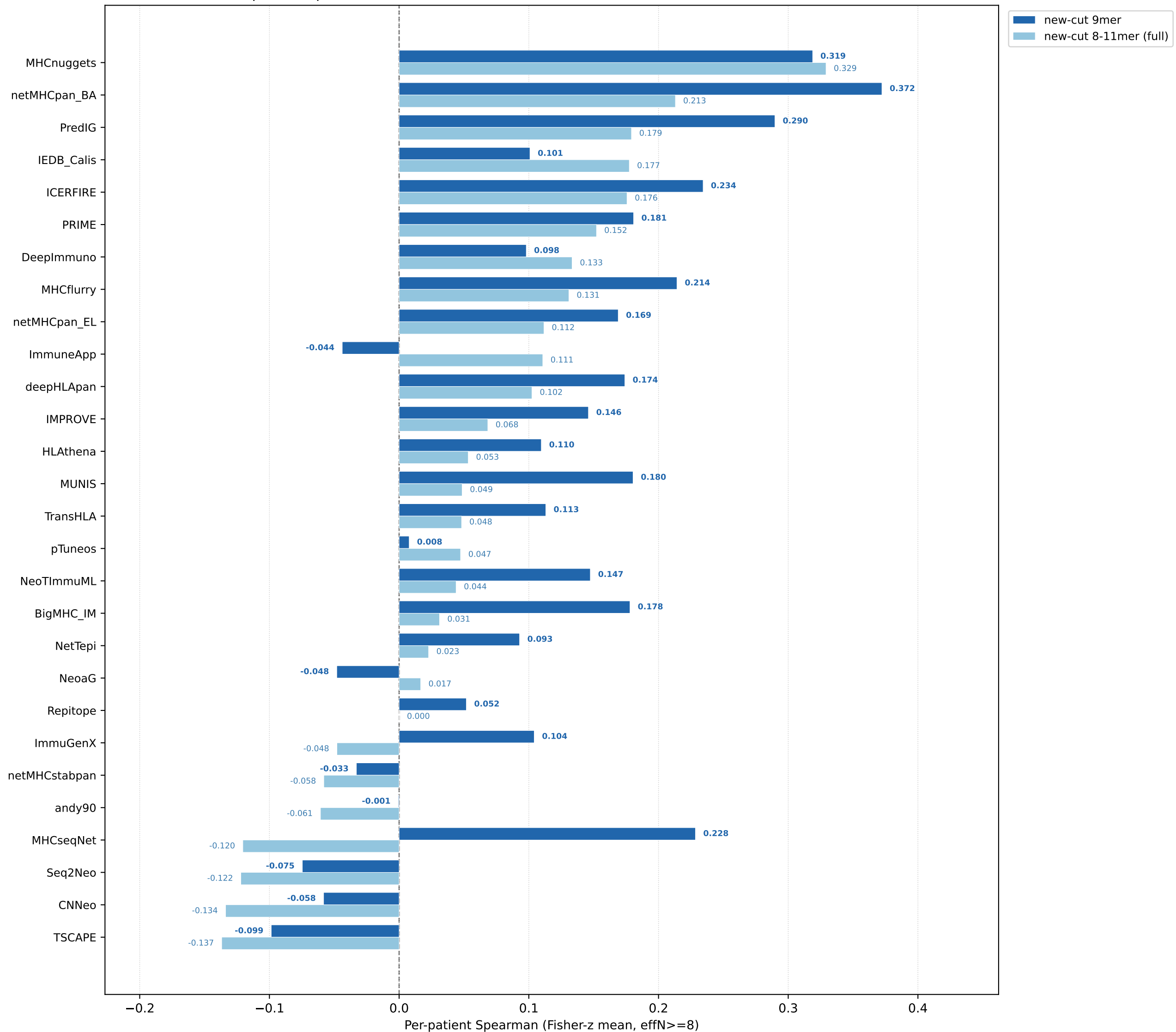
Per-patient Spearman: new-cut 9mer vs new-cut 8-11mer variable window (rerun, effN&gt;=8)
