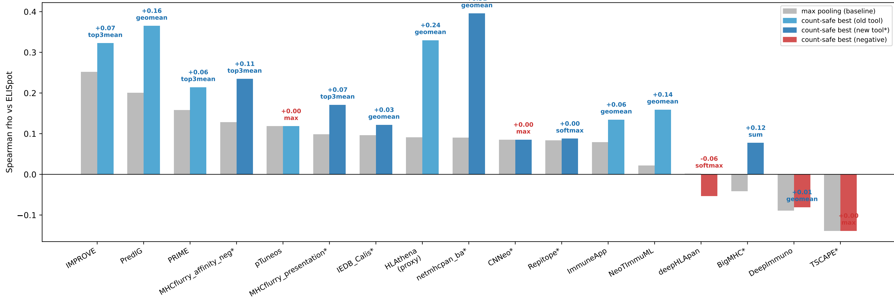
max pooling (baseline) vs Count-Safe Best Pooling, per Tool — 17 Tools Blue = uplift over max | Red = no signal after removing confounders
