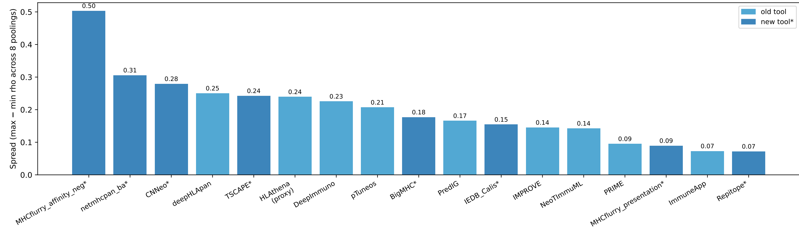
Pooling Sensitivity per Tool — 17 Tools Higher spread = more sensitive to pooling choice
