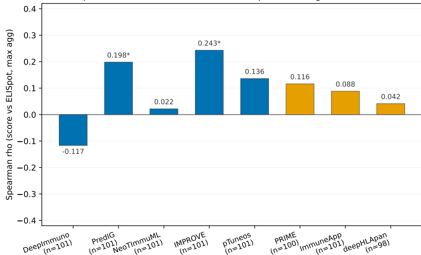
Per-tool Spearman correlation — all 8 tools (* p<0.05; magnitudes weak, near 0)
