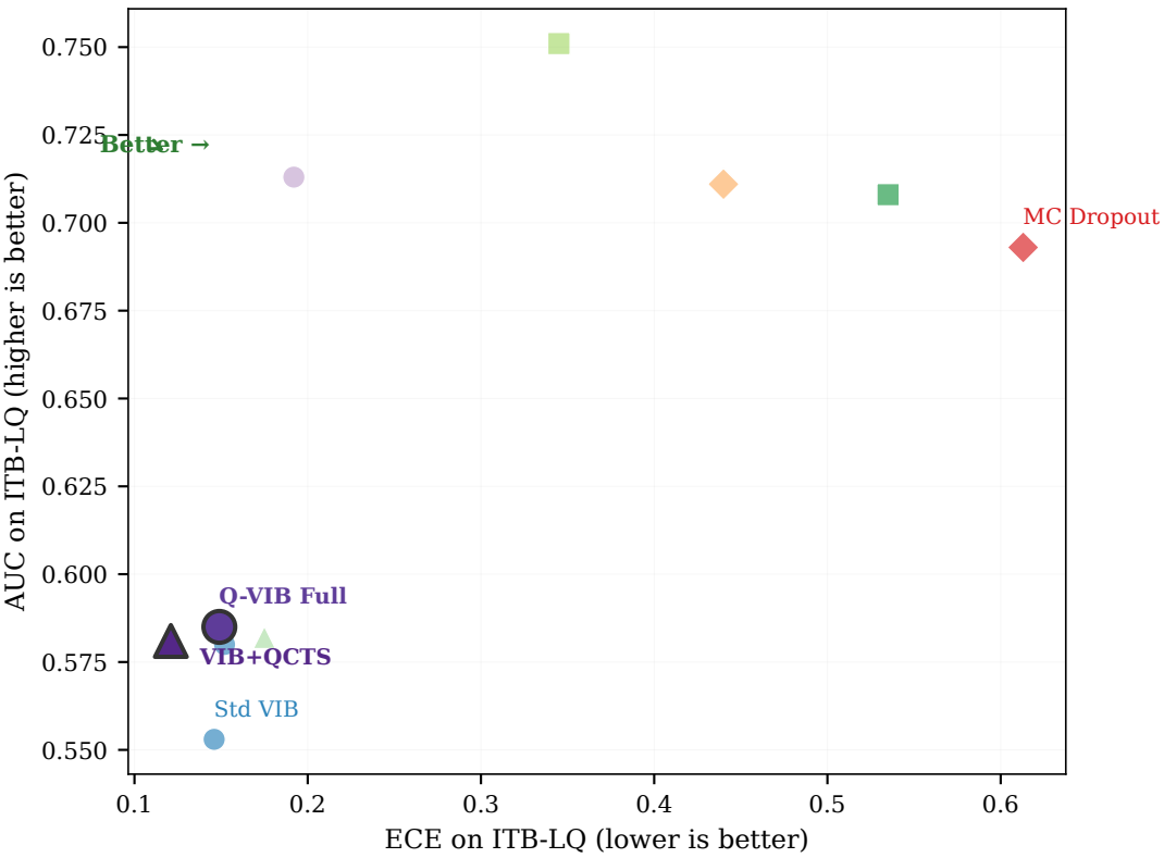
AUC-Calibration Trade-off on Low-Quality Images
