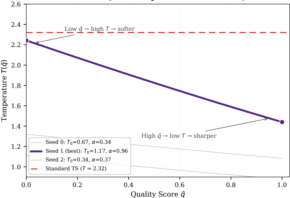
Learned QCTS Temperature Function T(\bar{q})
