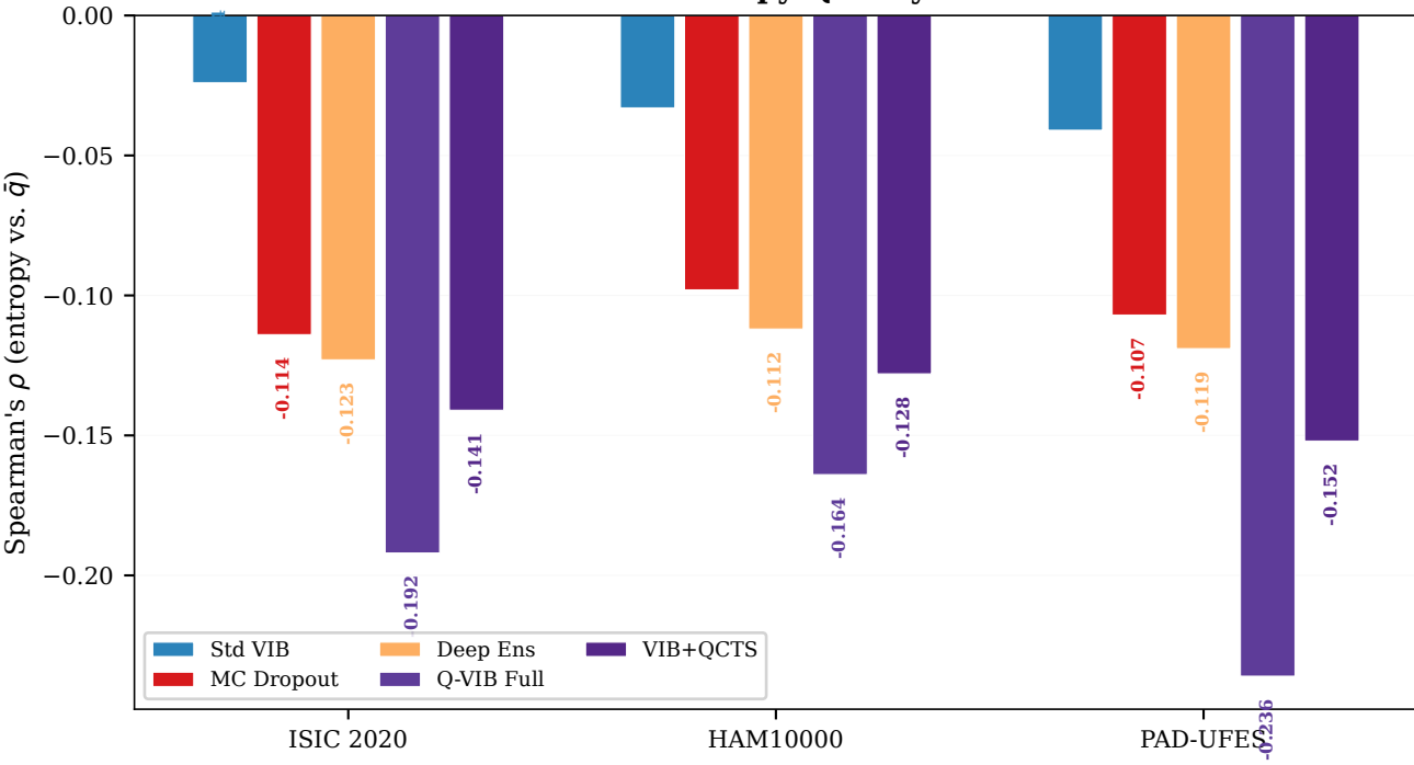
Cross-Dataset Entropy-Quality Correlation
