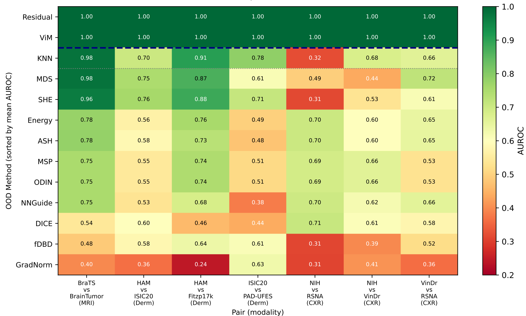
13-Method x 7-Pair AUROC Heatmap (cross-source normal-vs-normal, raw)
