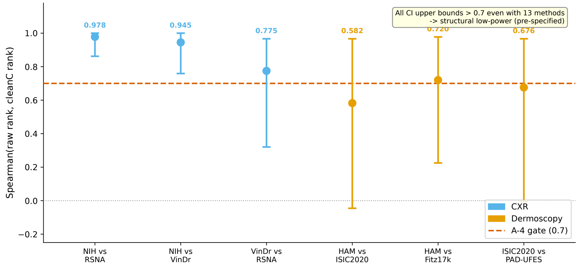
A-4 Negative Result: Ranking Correlation Raw vs Clean-C (6 evaluable pairs, 13 methods, 95% bootstrap CI)
