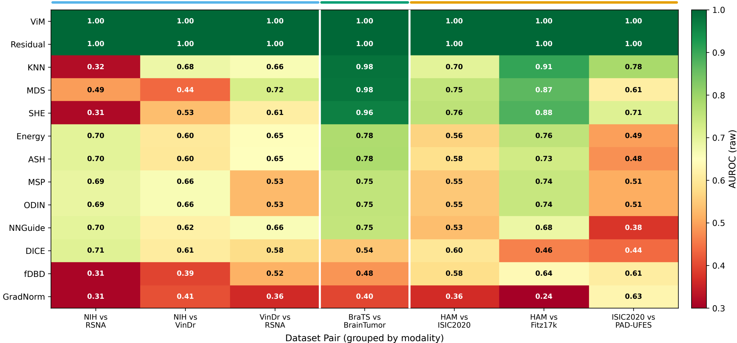
Artifact source-leakage across 13 OOD methods x 7 cross-source normal-vs-normal pairs
