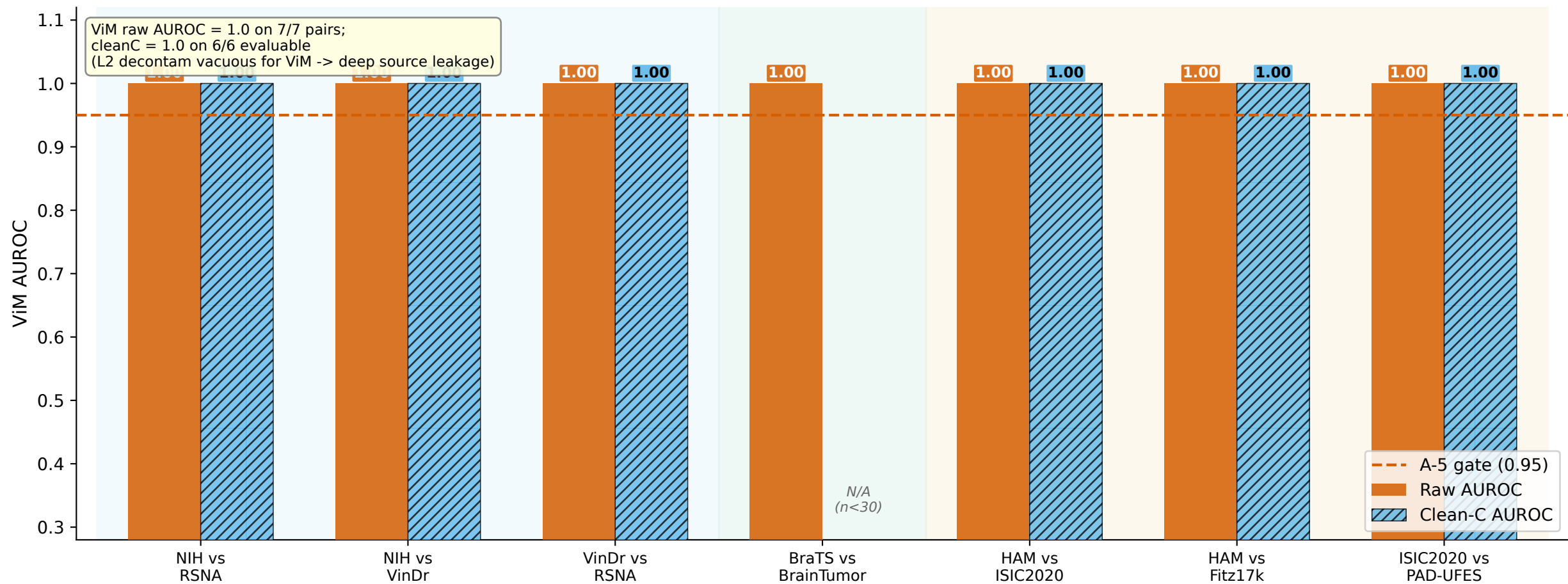
CXR ViM Source-Leakage: Raw vs Clean-C AUROC across 7 normal-vs-normal pairs Dermoscopy
