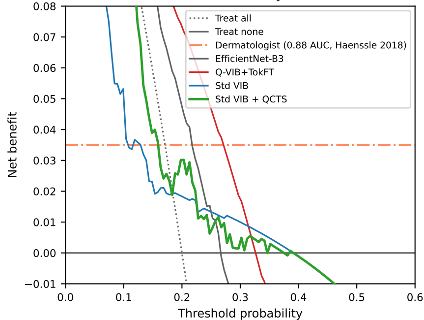
(a) Decision Curve Analysis (ITB-LQ)
