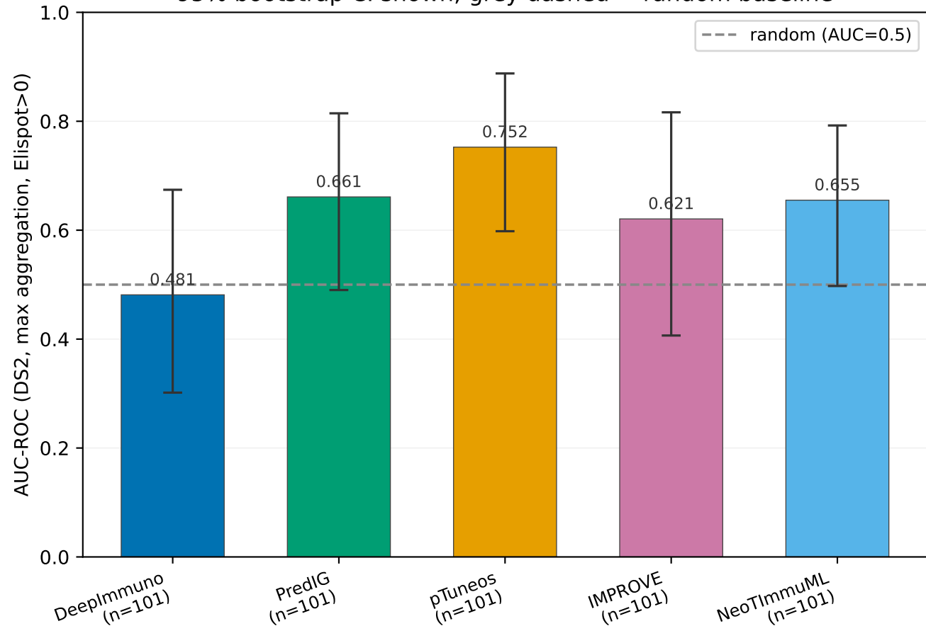
AUC-ROC — 5 first-batch tools (DS2, max agg, Elispot>0) 95% bootstrap CI shown; grey dashed = random baseline
