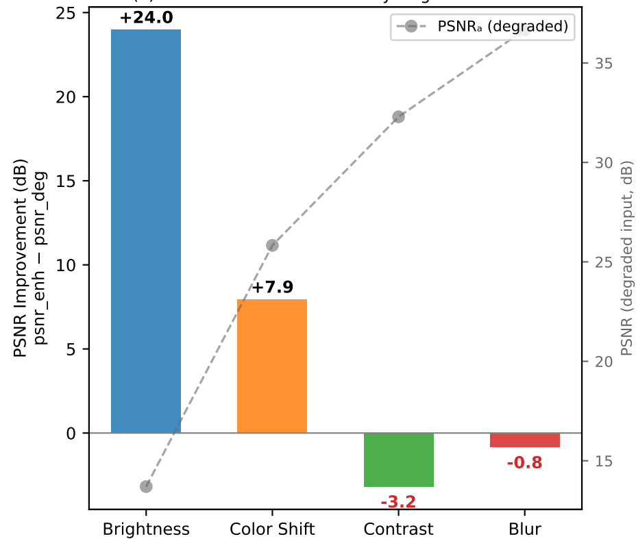
(a) Enhancement PSNR Gain by Degradation Axis
