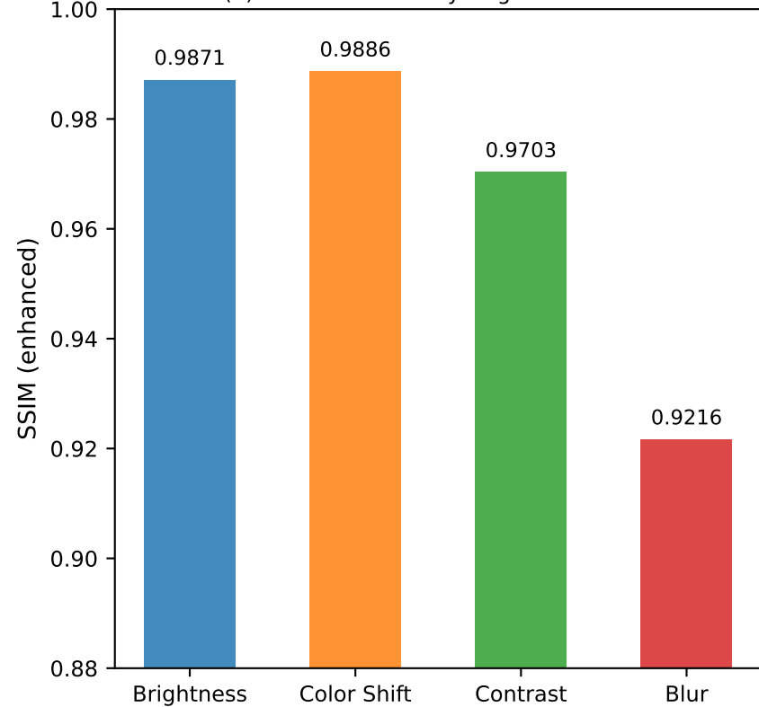
(b) Enhanced SSIM by Degradation Axis
